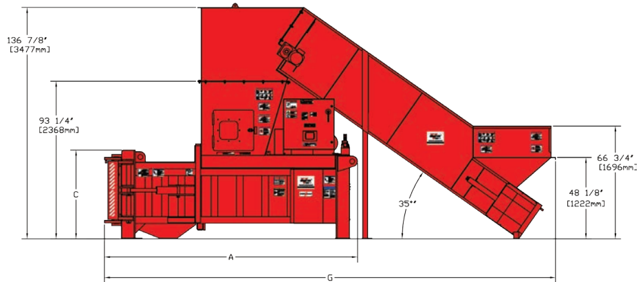
SIDE VIEW
